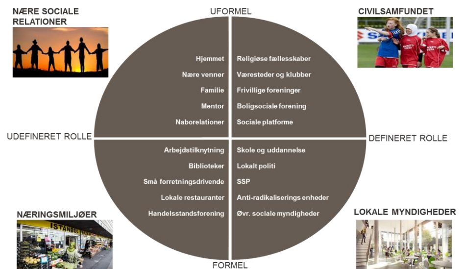
Figur 2: Datamodel
